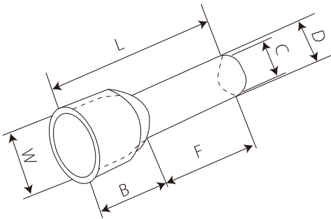
管形预绝缘端头 Insulated Cord End Terminals
