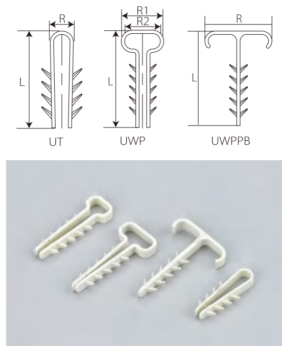
U型线类 U-type Cable Clamps
