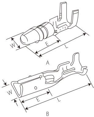
Open Barrel Terminals(female&male)
